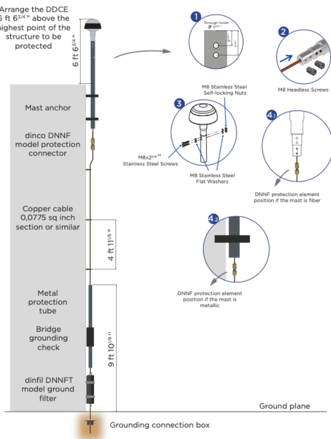
Figure 5. Installation of the DDCE Plus.
