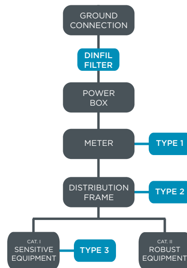
Figure 4. Electrical installation diagram.
